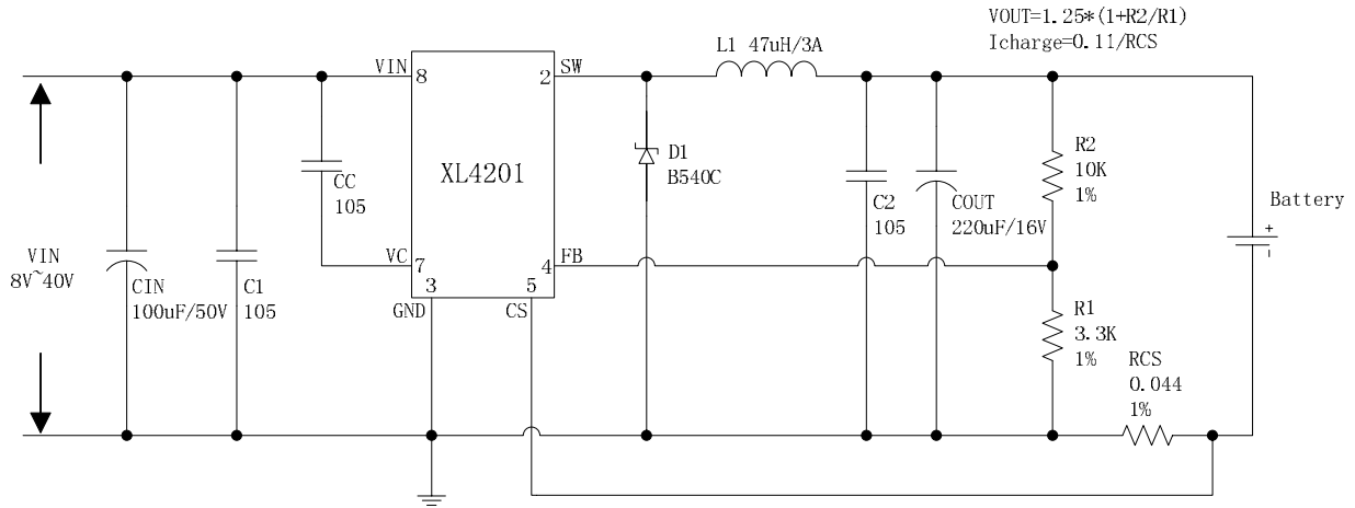
Figure6. XL4201 System Parameters Test Circuit (VIN=8V~40V, VOUT=5V/0.1A~2.5A)
